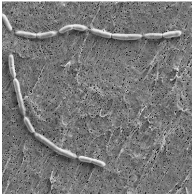
乳酸菌GR-1 ( Lactobacillus rhamnosus )
