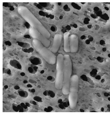
乳酸菌RC-14 ( Lactobacillus reuteri )
